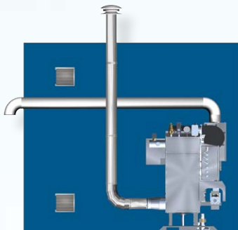
Direct Vent Unbalance Flue
