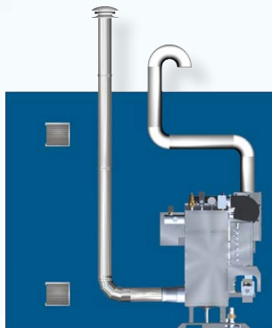
Direct Vent Vertical
